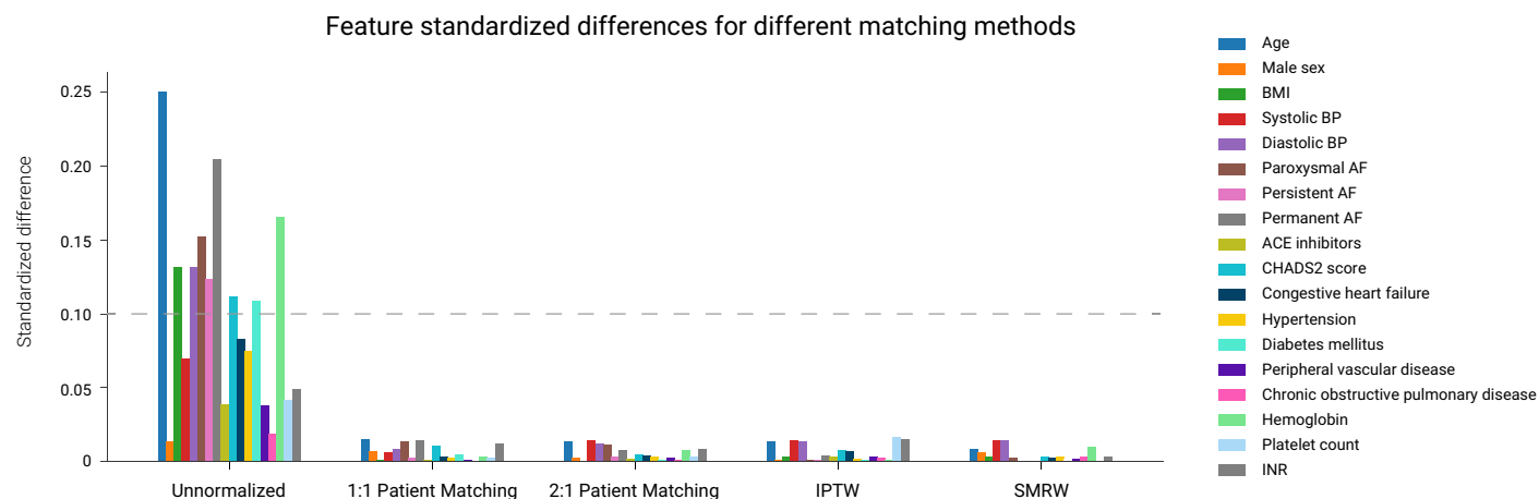
Figure 4. Standardized Differences across prognostic features for different matching methods: The standardized differences were calculated between rivaroxaban and warfarin cohorts prior to balancing (Unnormalized) and for each balancing method. The standardized difference was dramatically reduced using all of the methods explored, with SMRW showing the largest decrease in average standardized difference.
