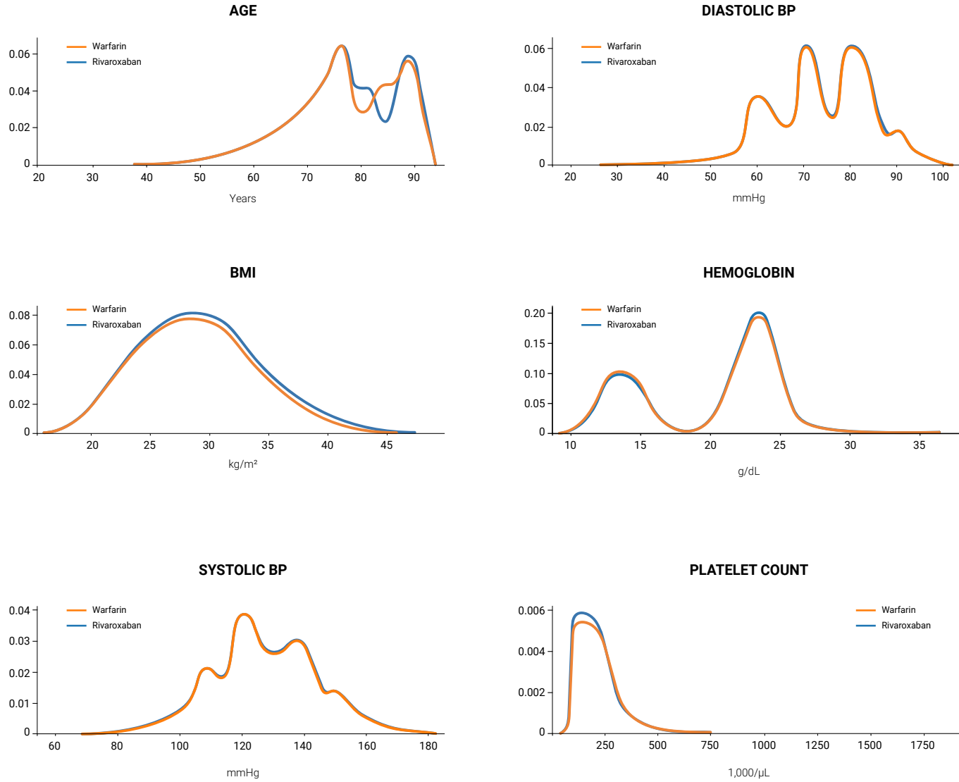
Figure 5. Histograms of continuous variables after weighting using SMRW.
